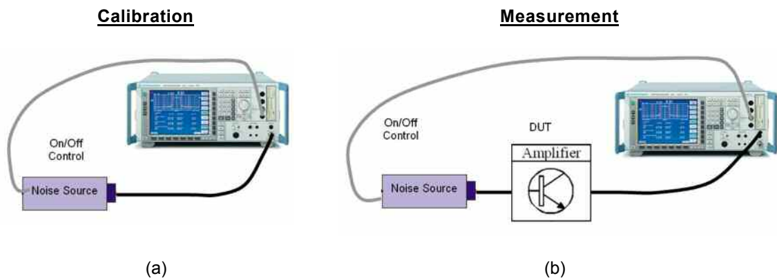
Figure 5: Connection diagram for (a) the calibration step, and (b) the measurement of the DUT's noise figure.
