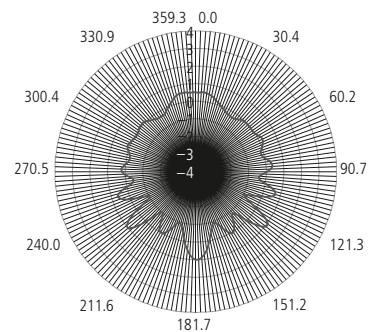
Typical ripple with dipole, average normalized (1880 MHz)
